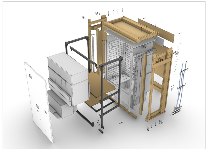
Exploded view of a Katerra Bath Kit.
